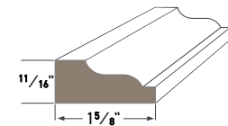
Shingle Moulding AZM-210 Length: 16'
