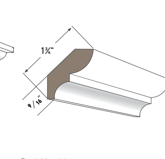
Bed Moulding AZM-75 Length: 16'
